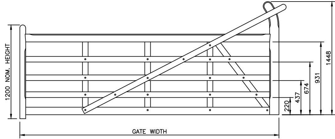
VIEWED FROM OUTSIDE GATE RIGHT HAND HANGING. (AUTOMATED)
