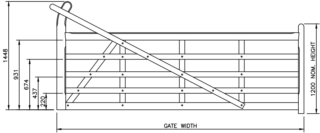
VIEWED FROM OUTSIDE GATE LEFT HAND HANGING. (AUTOMATED)
